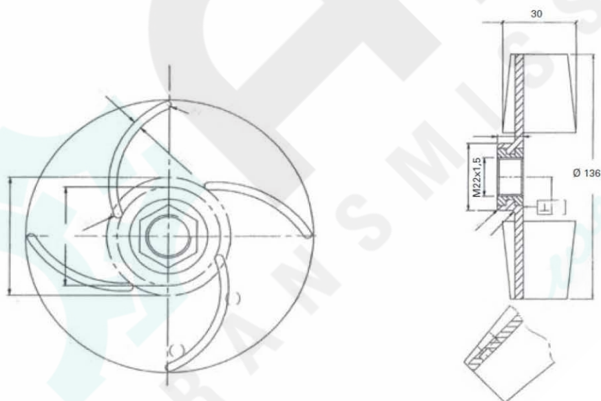
Girante SX per pompa – Pale ribassate Left plastic fan with flaps lowered Turbina SX rebajada para bomba
