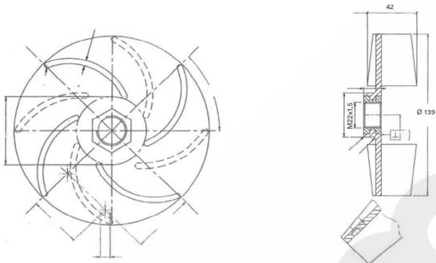
Girante SX per pompa Left plastic fan with high flaps Turbina SX para bomba
